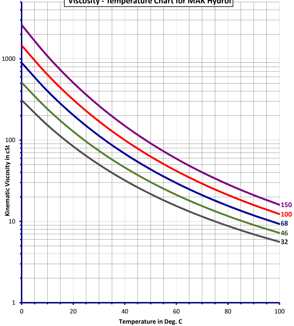
Viscosity - Temperature Chart for MAK Hydrol
